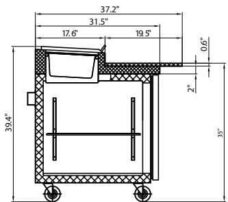
SECTION VIEW
