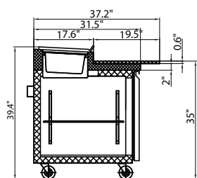
SECTION VIEW
